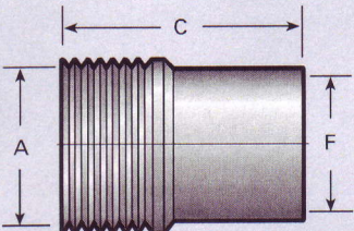
Male Adapter
